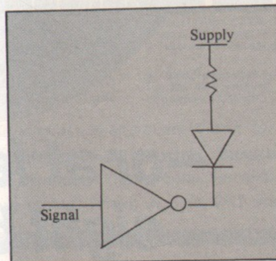
Figure IV: LED driven from buffer
