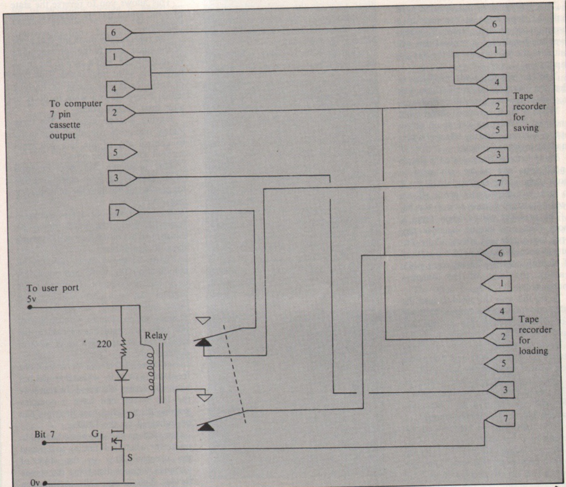
Figure VIII: Dual cassette system
