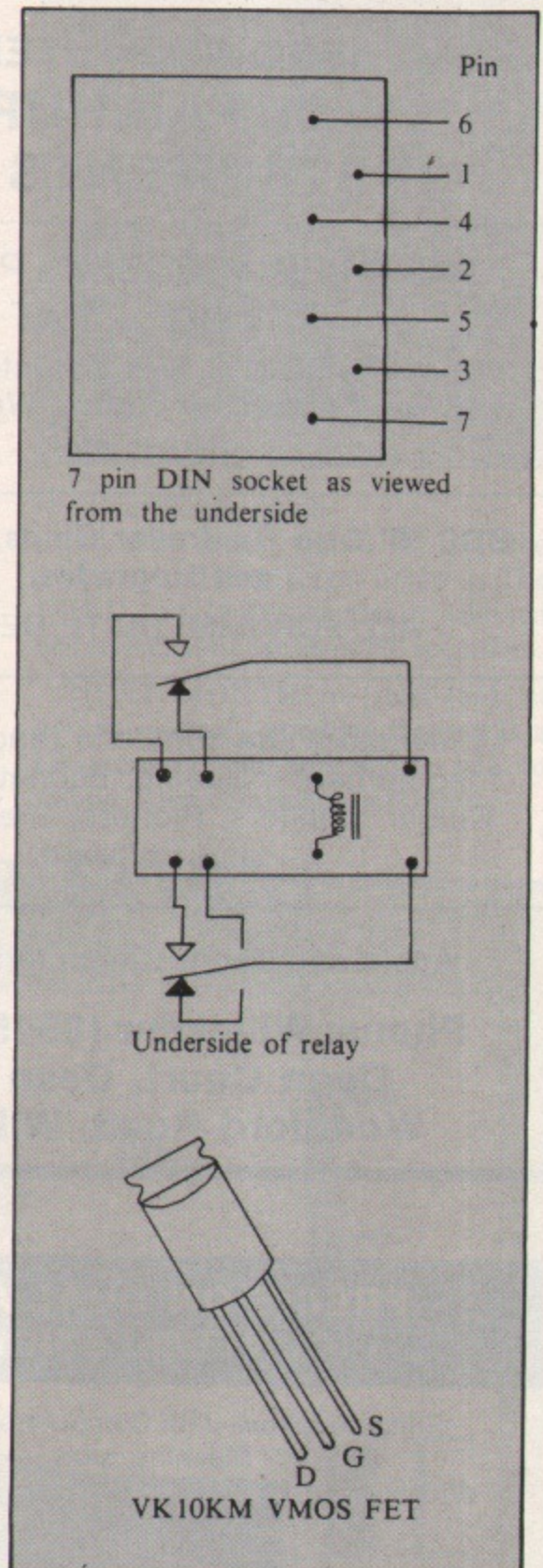
Figure IX: Component pinout
