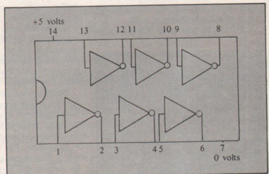
Figure V: Pinout of 74LS05 buffer
