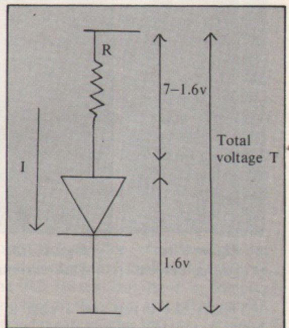
Figure 1: Voltage and currents on an LED
